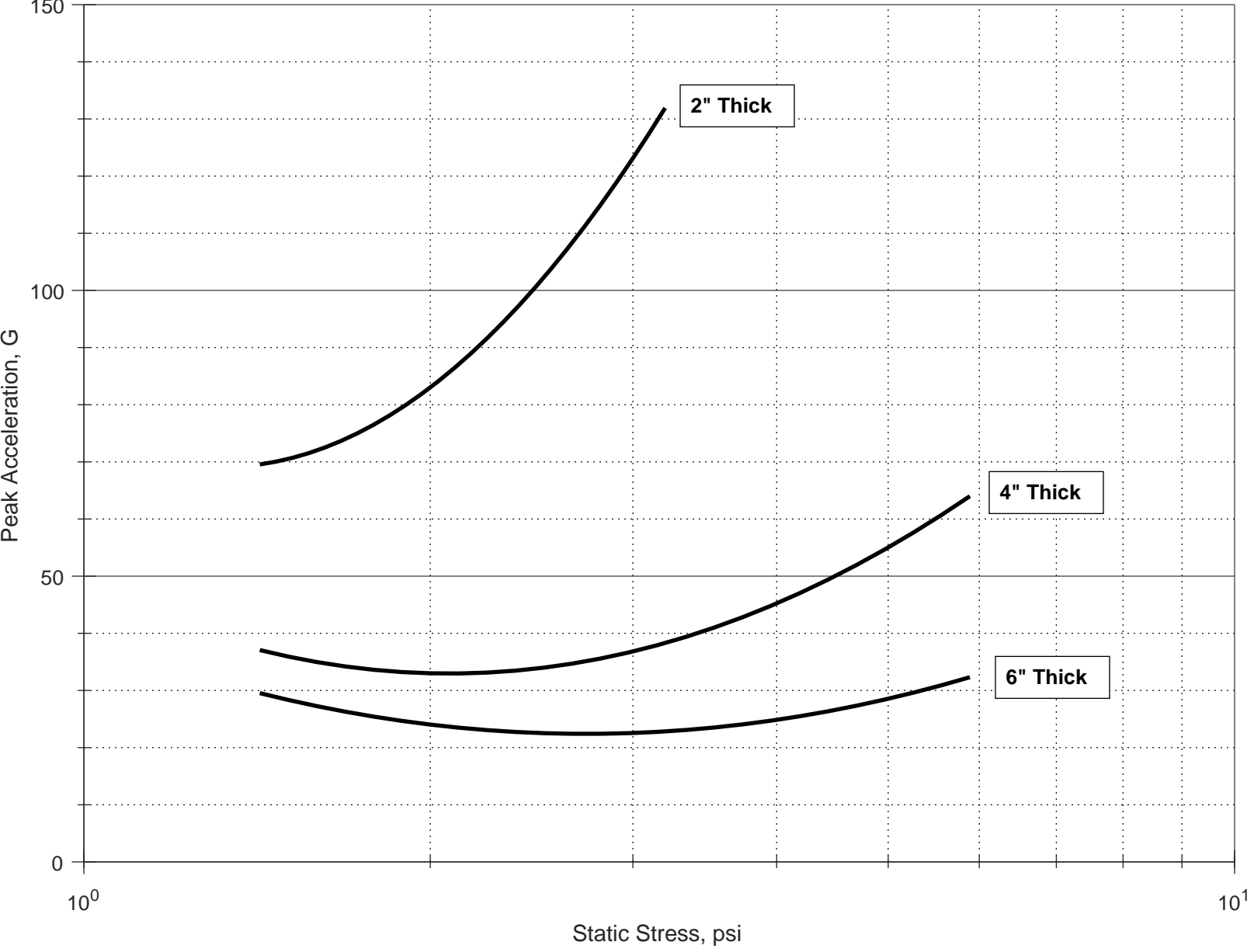
Peak Acceleration vs. Static Stress, Type 5 PE Foam, 36" Drop Height, 140 deg F
