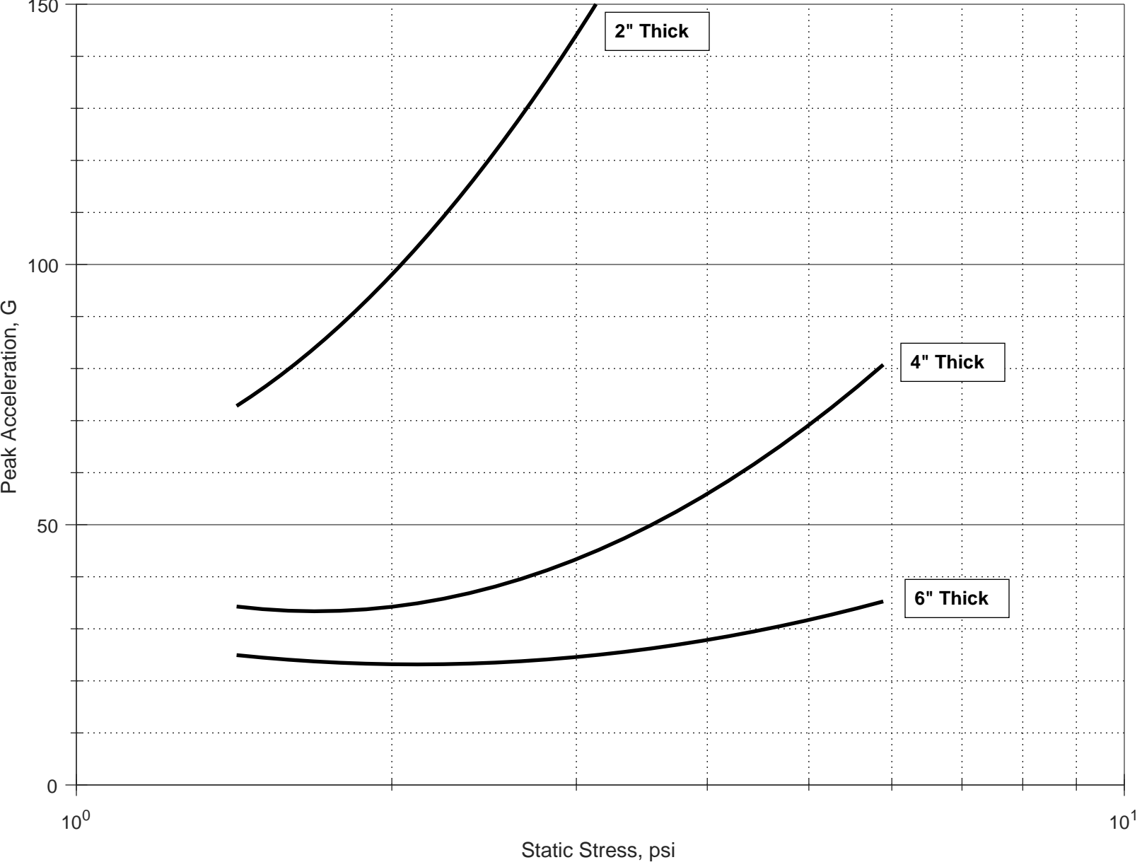
Peak Acceleration vs. Static Stress, Type 5 PE Foam, 36" Drop Height, 160 deg F
