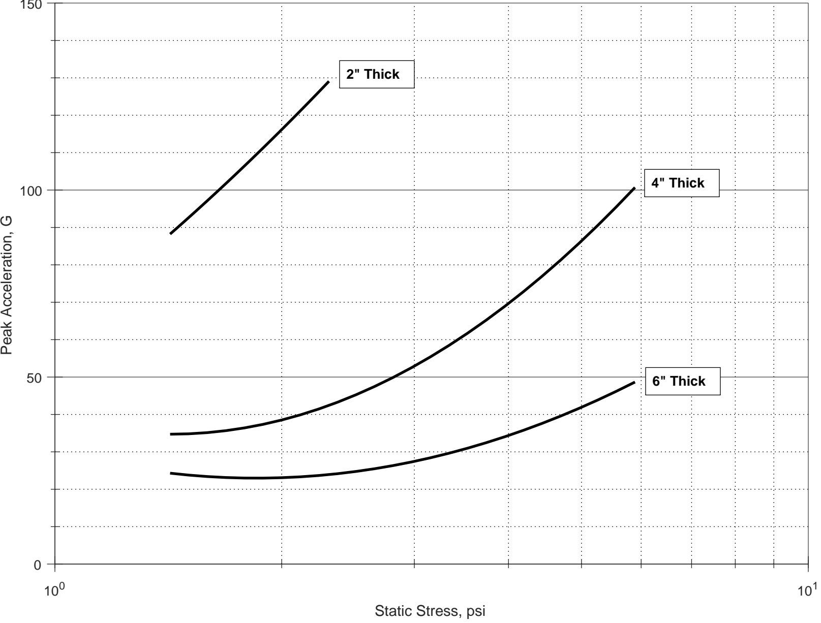
Peak Acceleration vs. Static Stress, Type 5 PE Foam, 36" Drop Height, 180 deg F
