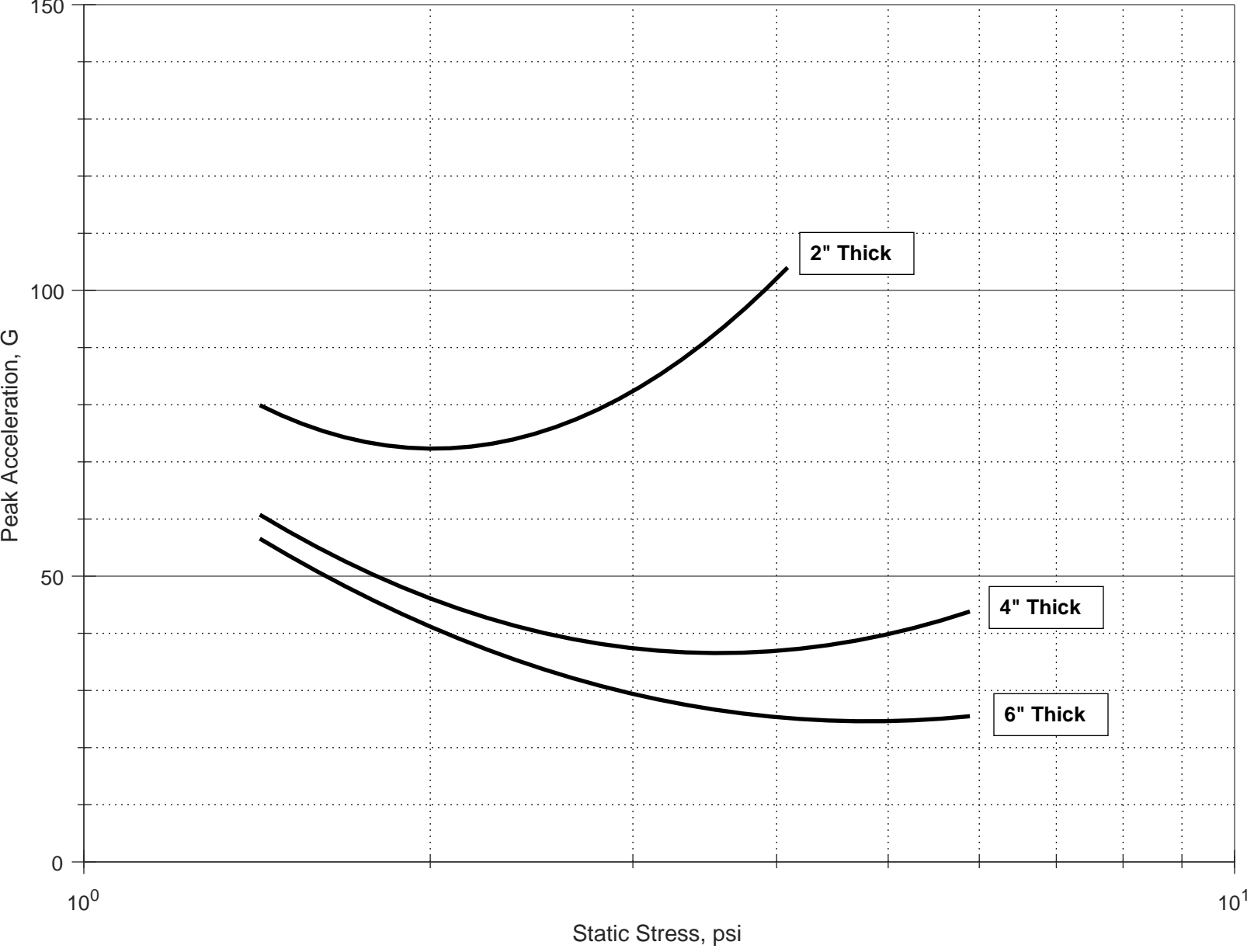
Peak Acceleration vs. Static Stress, Type 5 PE Foam, 36" Drop Height, 73 deg F
