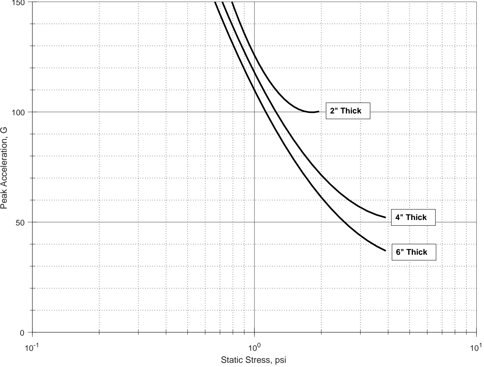
Peak Acceleration vs. Static Stress, Type 4 PE Foam, 36" Drop Height, -65 deg F
