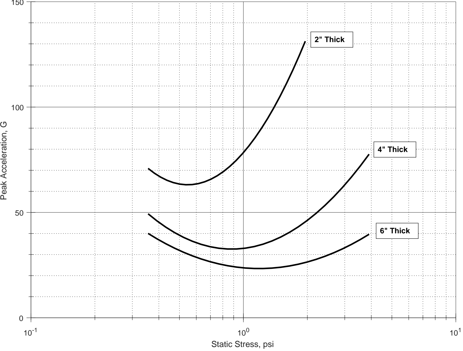
Peak Acceleration vs. Static Stress, Type 4 PE Foam, 36" Drop Height, 140 deg F
