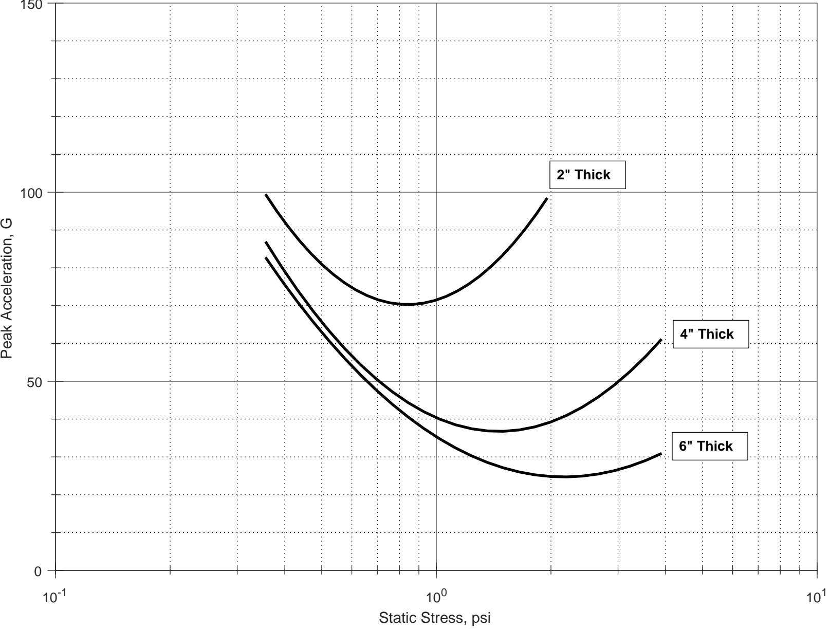
Peak Acceleration vs. Static Stress, Type 4 PE Foam, 36" Drop Height, 73 deg F
