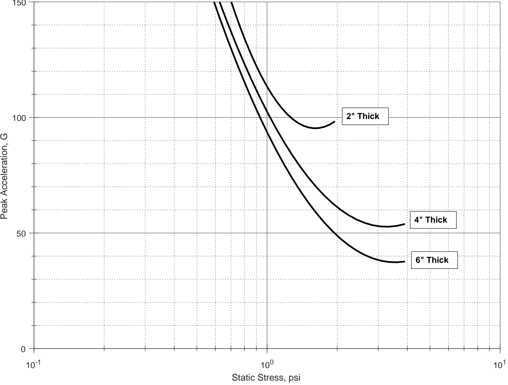
Peak Acceleration vs. Static Stress, Type 4 PE Foam, 36" Drop Height, -40 deg F
