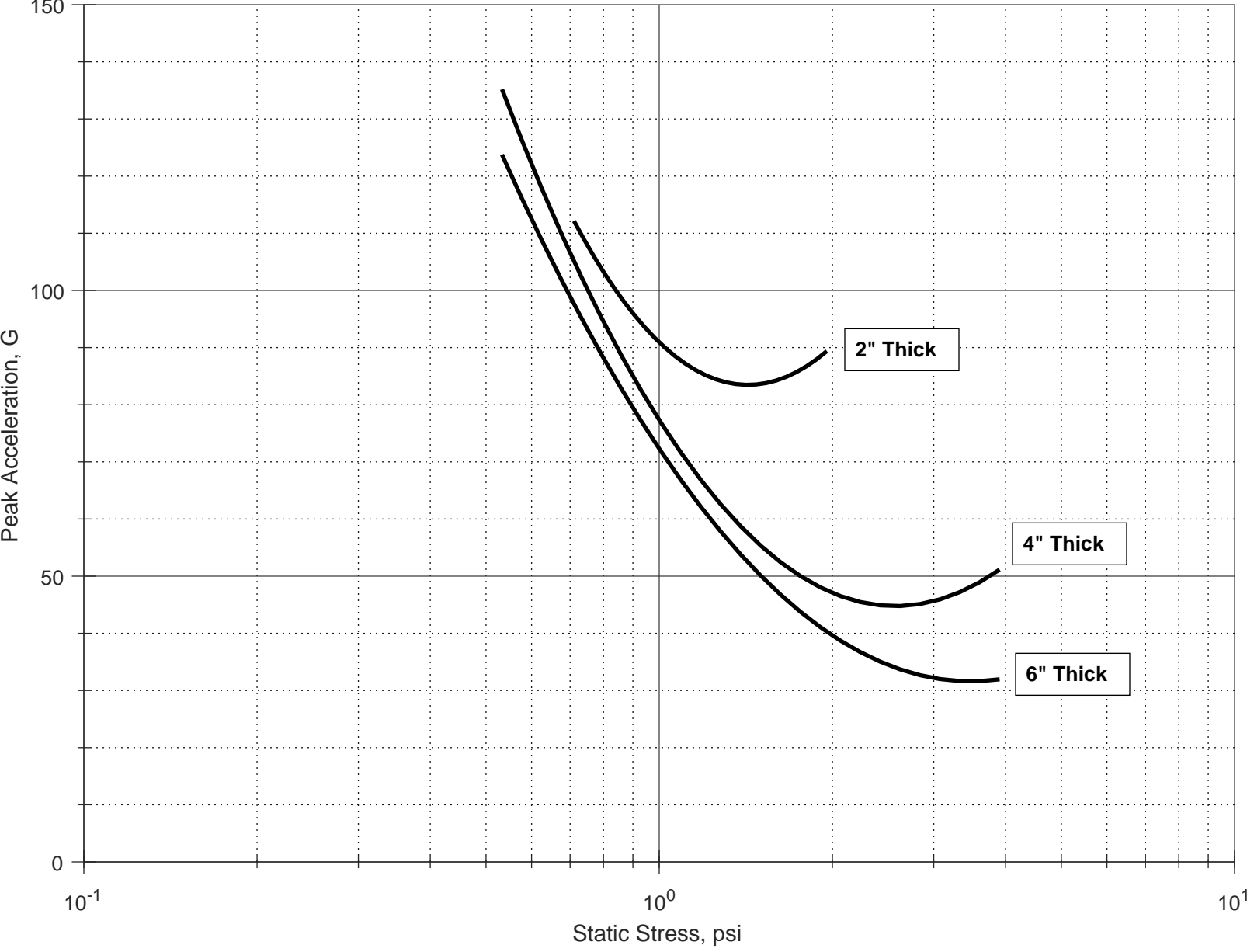
Peak Acceleration vs. Static Stress, Type 4 PE Foam, 36" Drop Height, 0 deg F
