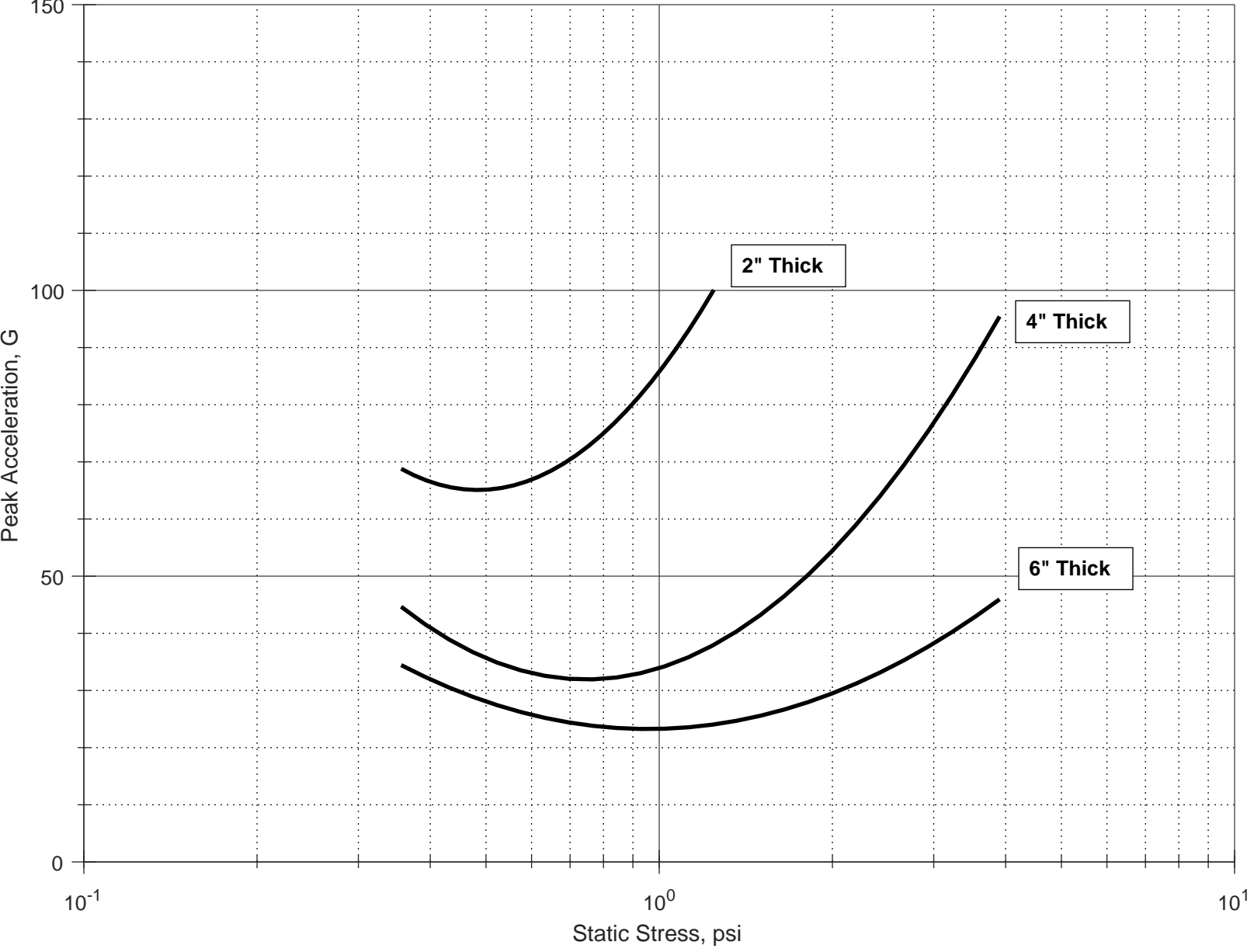
Peak Acceleration vs. Static Stress, Type 4 PE Foam, 36" Drop Height, 160 deg F
