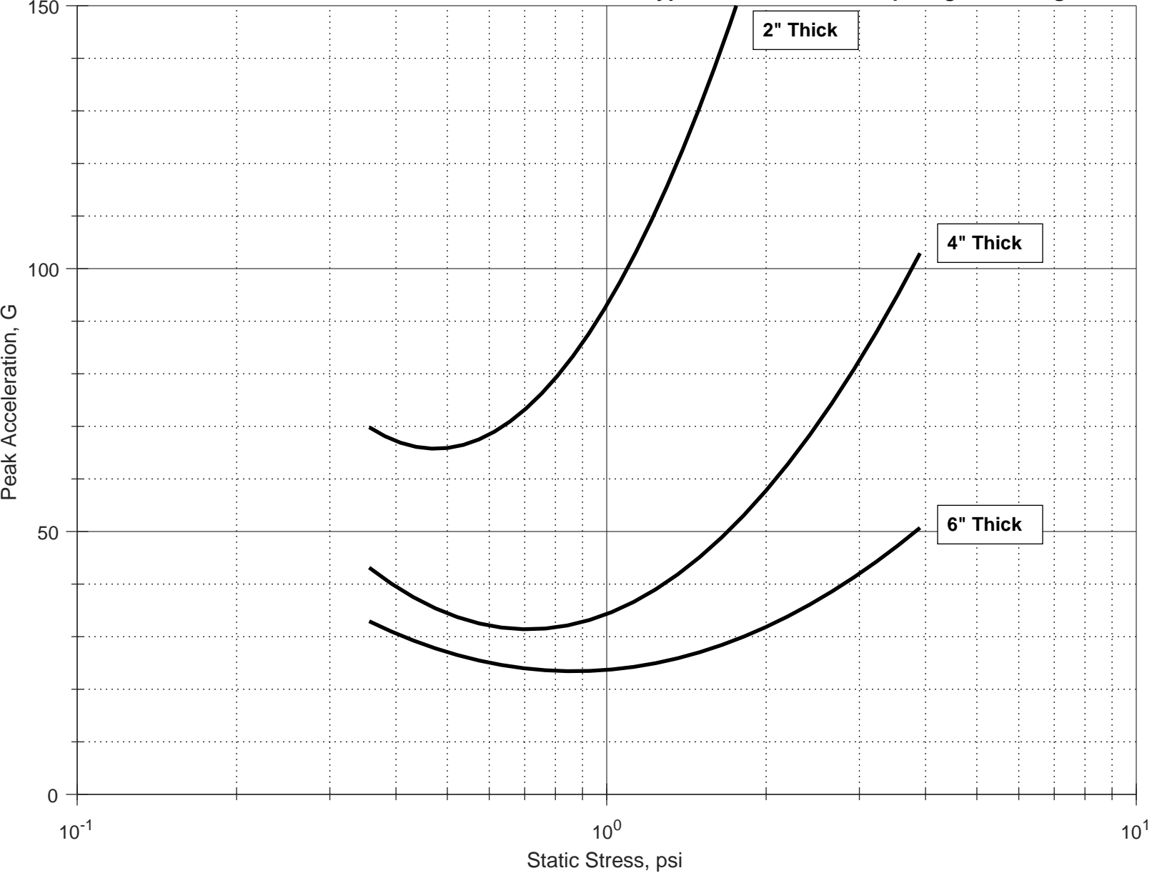
Peak Acceleration vs. Static Stress, Type 4 PE Foam, 36" Drop Height, 180 deg F
