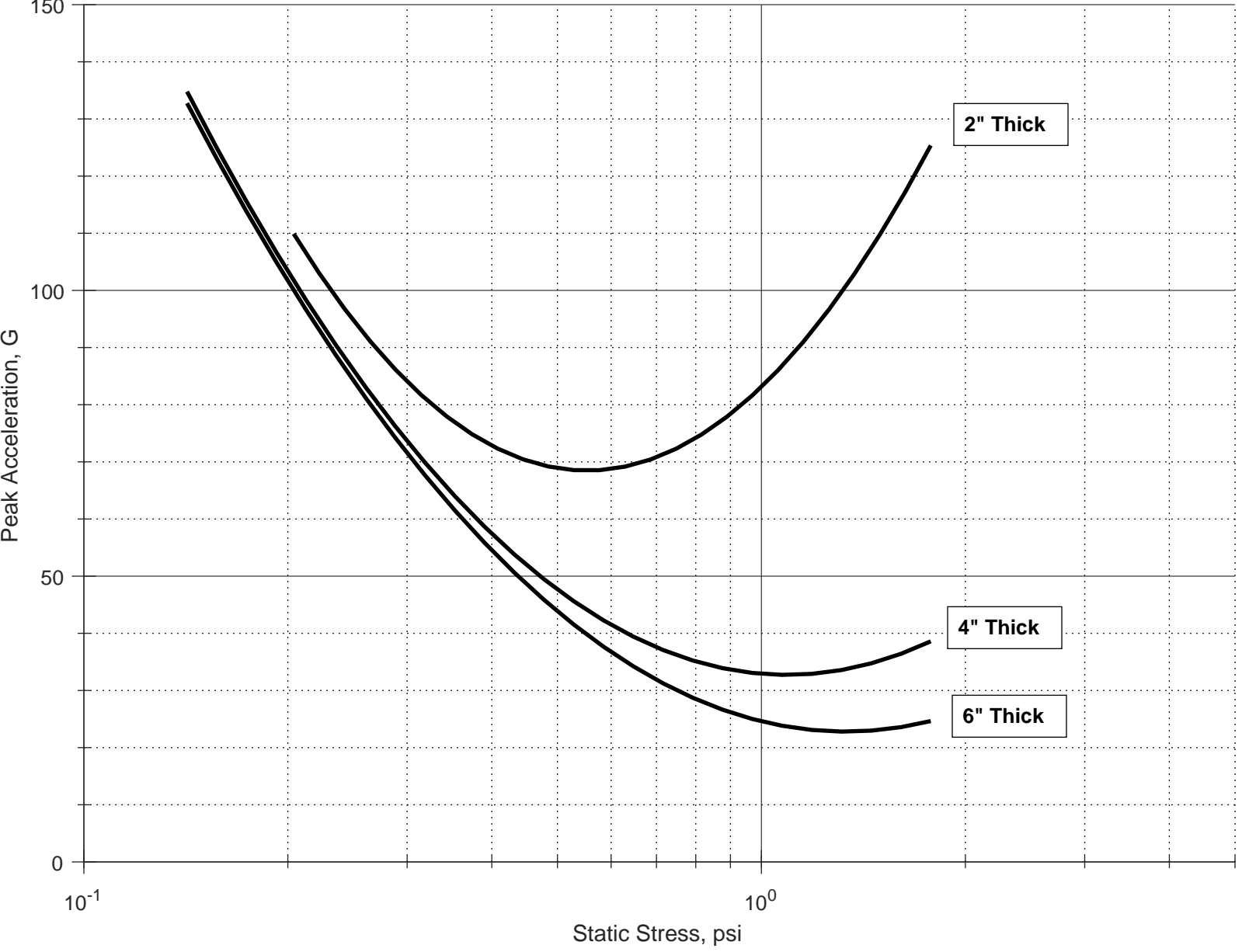
Peak Acceleration vs. Static Stress, Type 3 PE Foam, 36" Drop Height, 73 deg F
