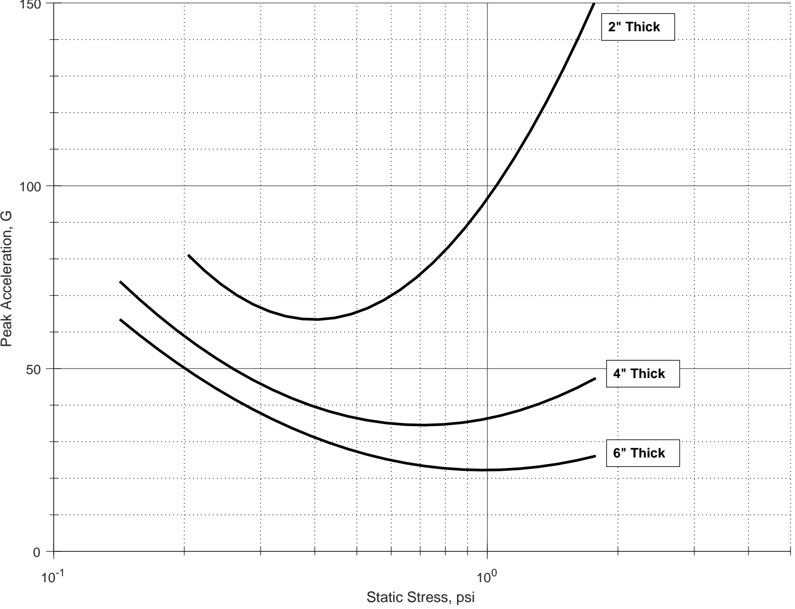
Peak Acceleration vs. Static Stress, Type 3 PE Foam, 36" Drop Height, 140 deg F
