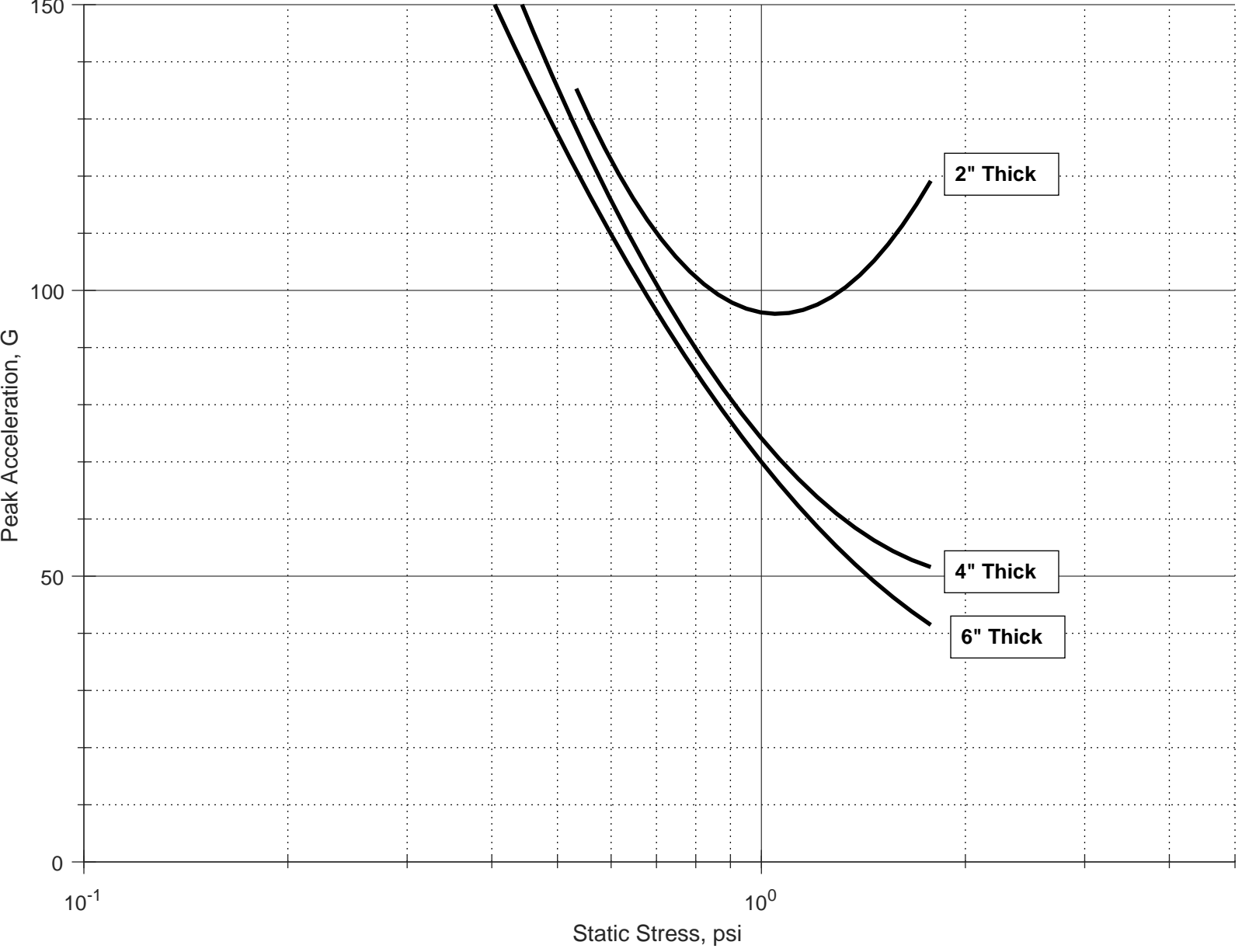
Peak Acceleration vs. Static Stress, Type 3 PE Foam, 36" Drop Height, -40 deg F
