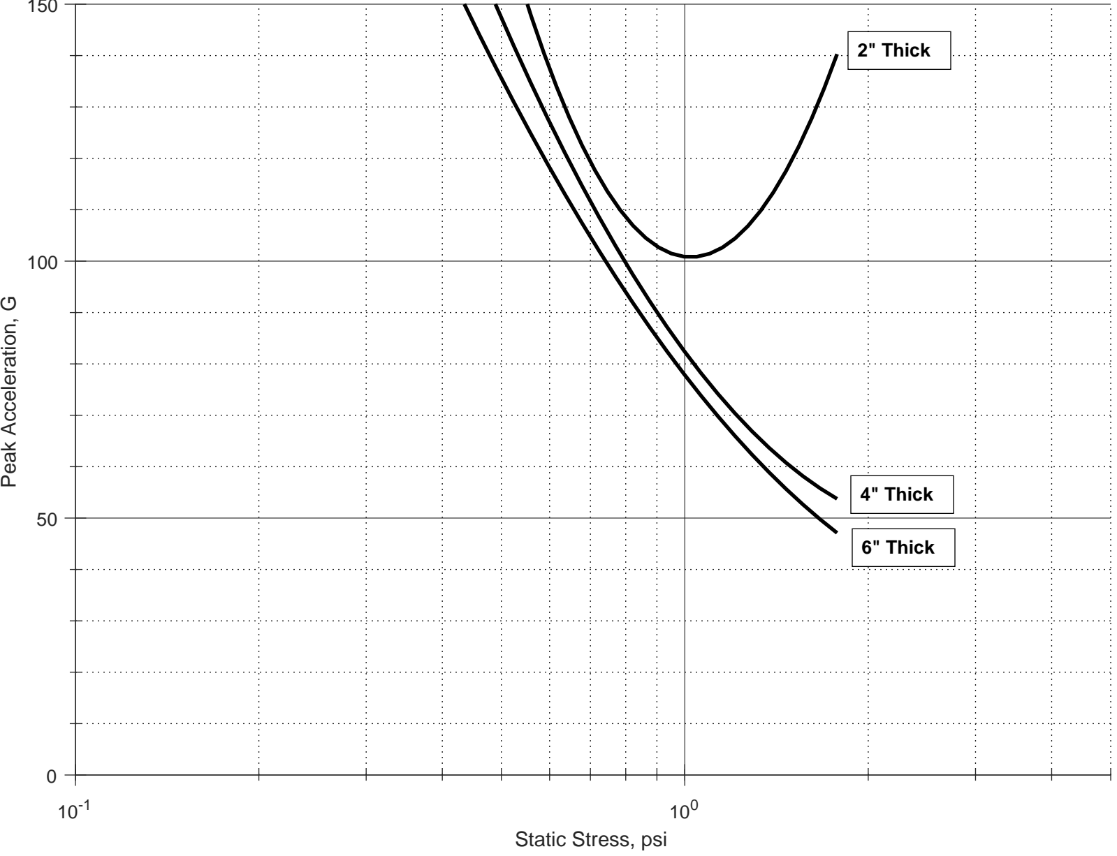
Peak Acceleration vs. Static Stress, Type 3 PE Foam, 36" Drop Height, -65 deg F
