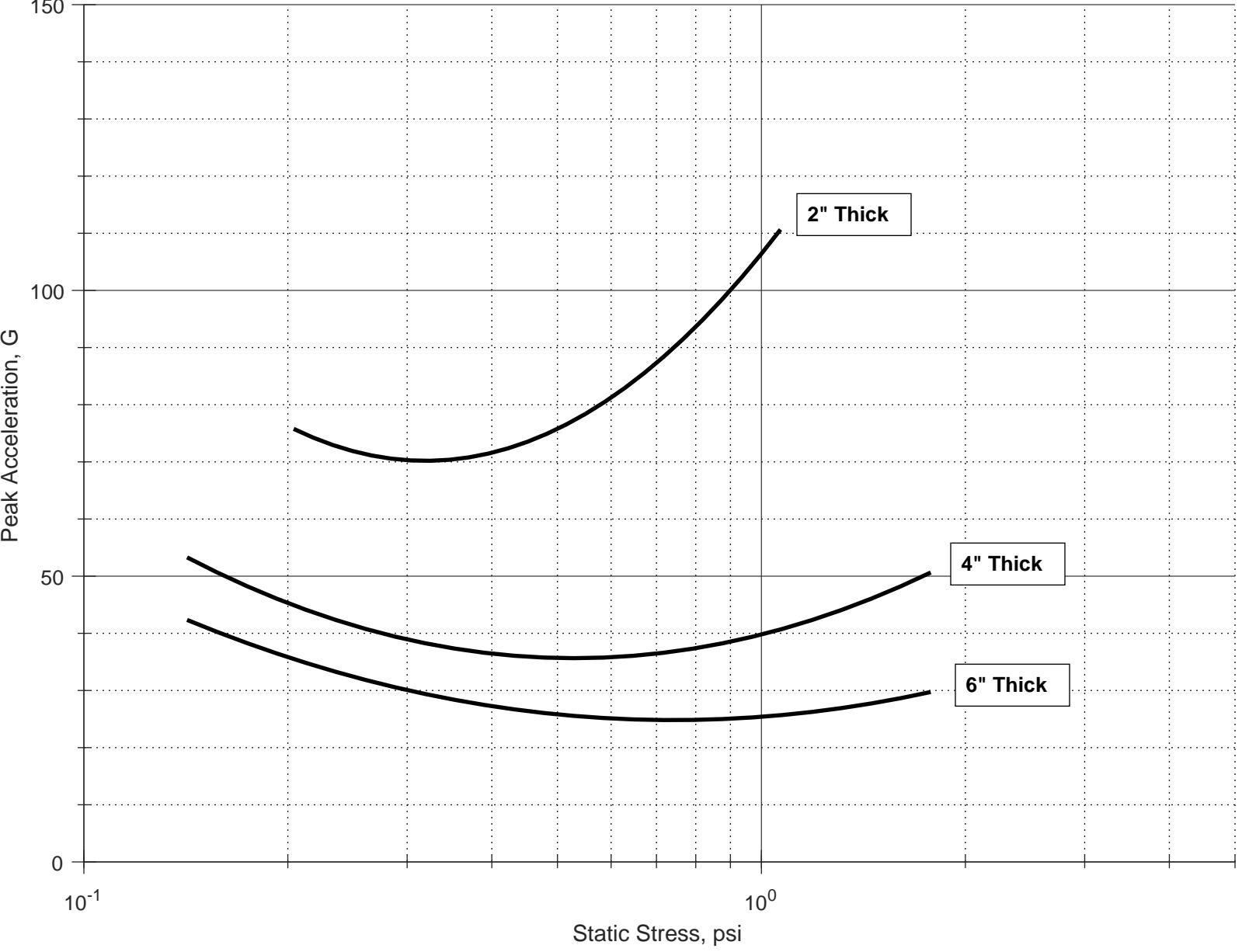
Peak Acceleration vs. Static Stress, Type 3 PE Foam, 36" Drop Height, 180 deg F
