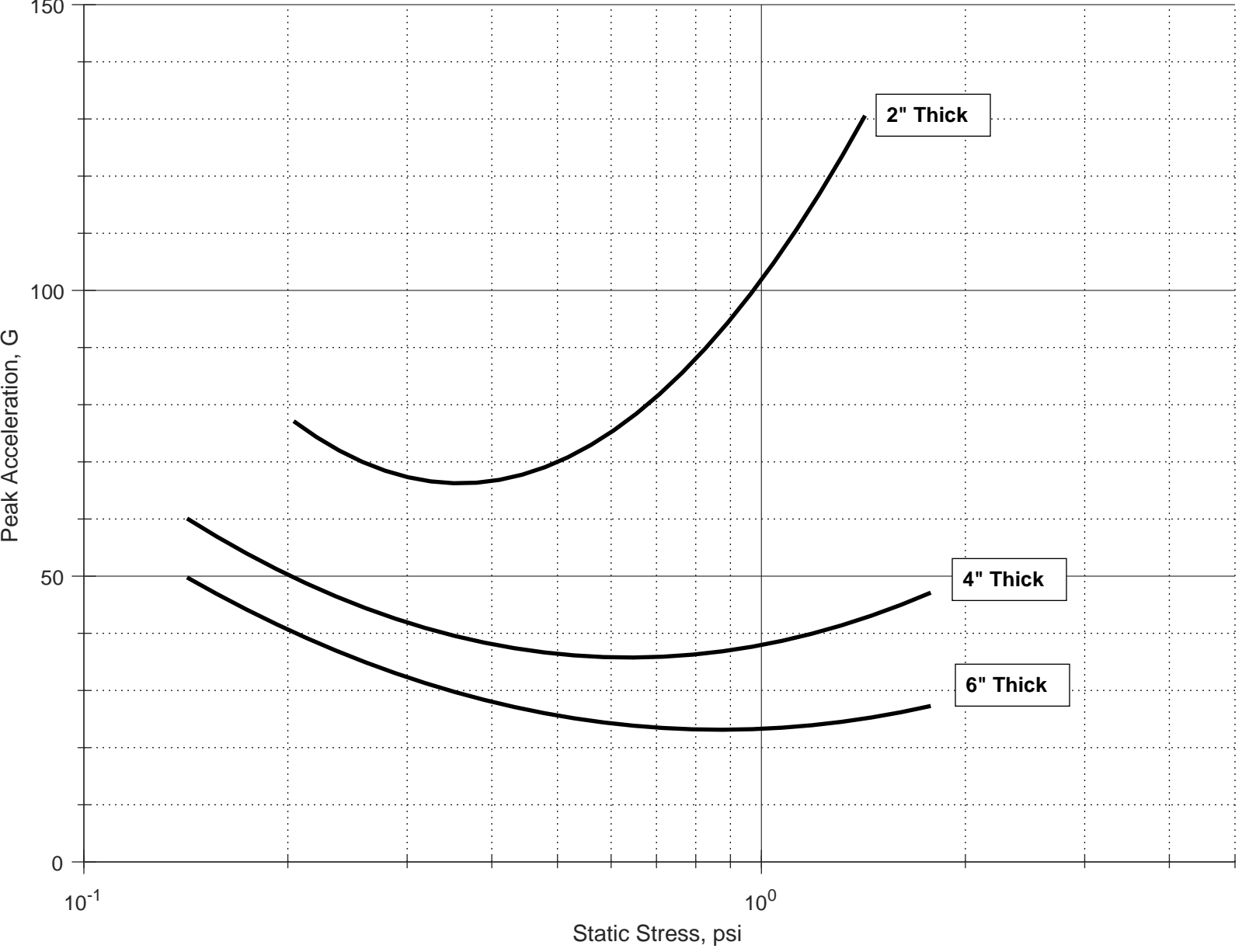
Peak Acceleration vs. Static Stress, Type 3 PE Foam, 36" Drop Height, 160 deg F
