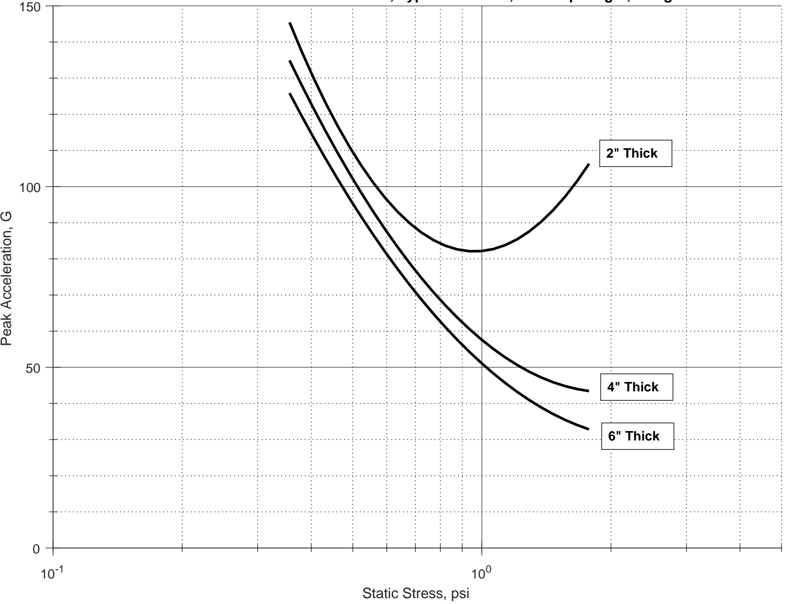
Peak Acceleration vs. Static Stress, Type 3 PE Foam, 36" Drop Height, 0 deg F
