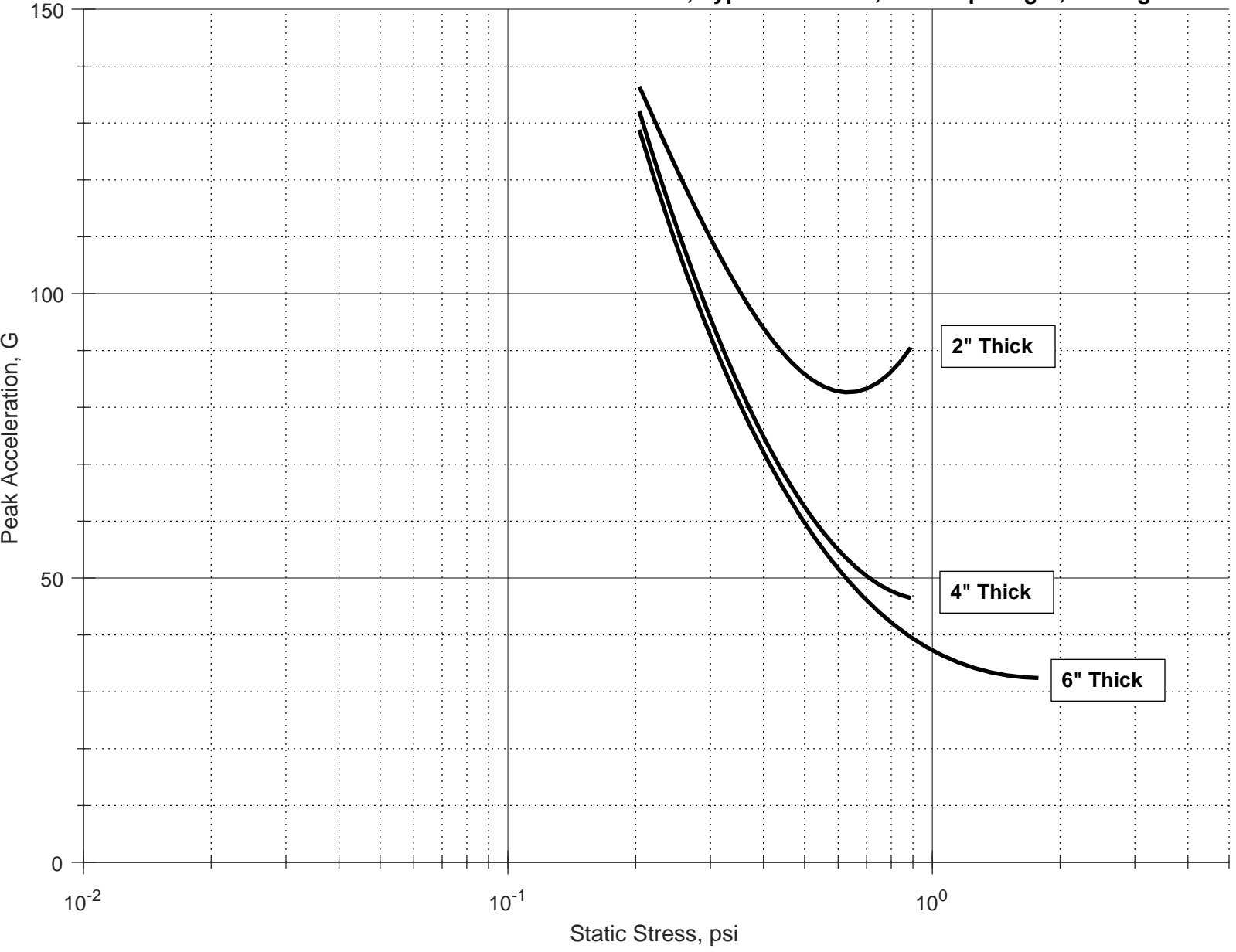
Peak Acceleration vs. Static Stress, Type 1 PE Foam, 36" Drop Height, -40 deg F
