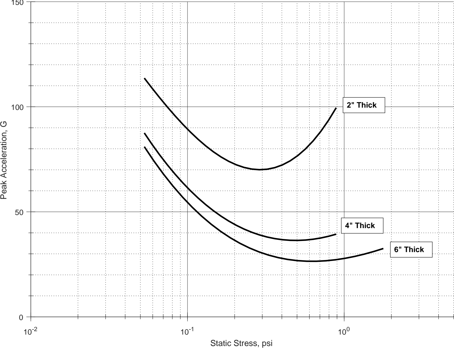
Peak Acceleration vs. Static Stress, Type 1 PE Foam, 36" Drop Height, 140 deg F
