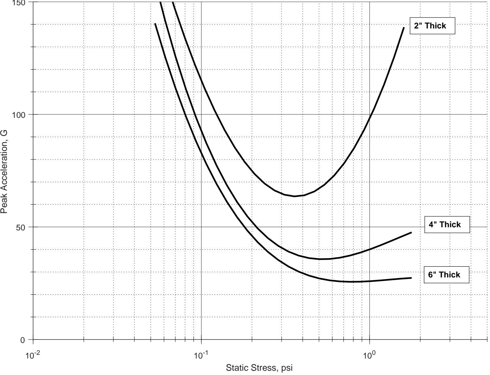
Peak Acceleration vs. Static Stress, Type 1 PE Foam, 36" Drop Height, 73 deg F
