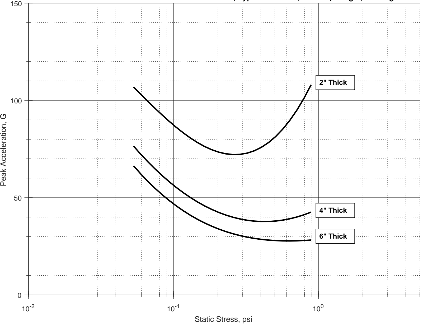
Peak Acceleration vs. Static Stress, Type 1 PE Foam, 36" Drop Height, 160 deg F
