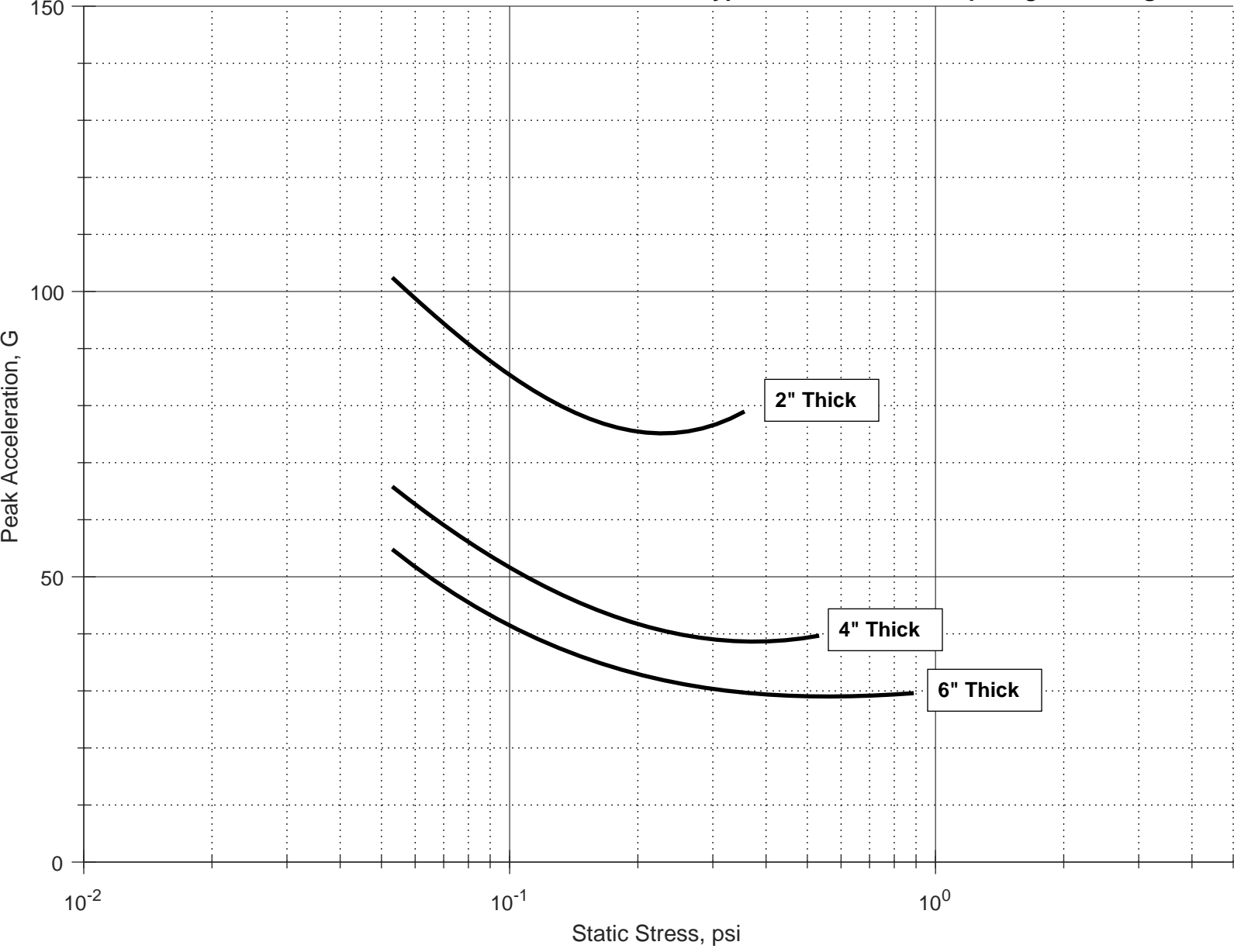
Peak Acceleration vs. Static Stress, Type 1 PE Foam, 36" Drop Height, 180 deg F
