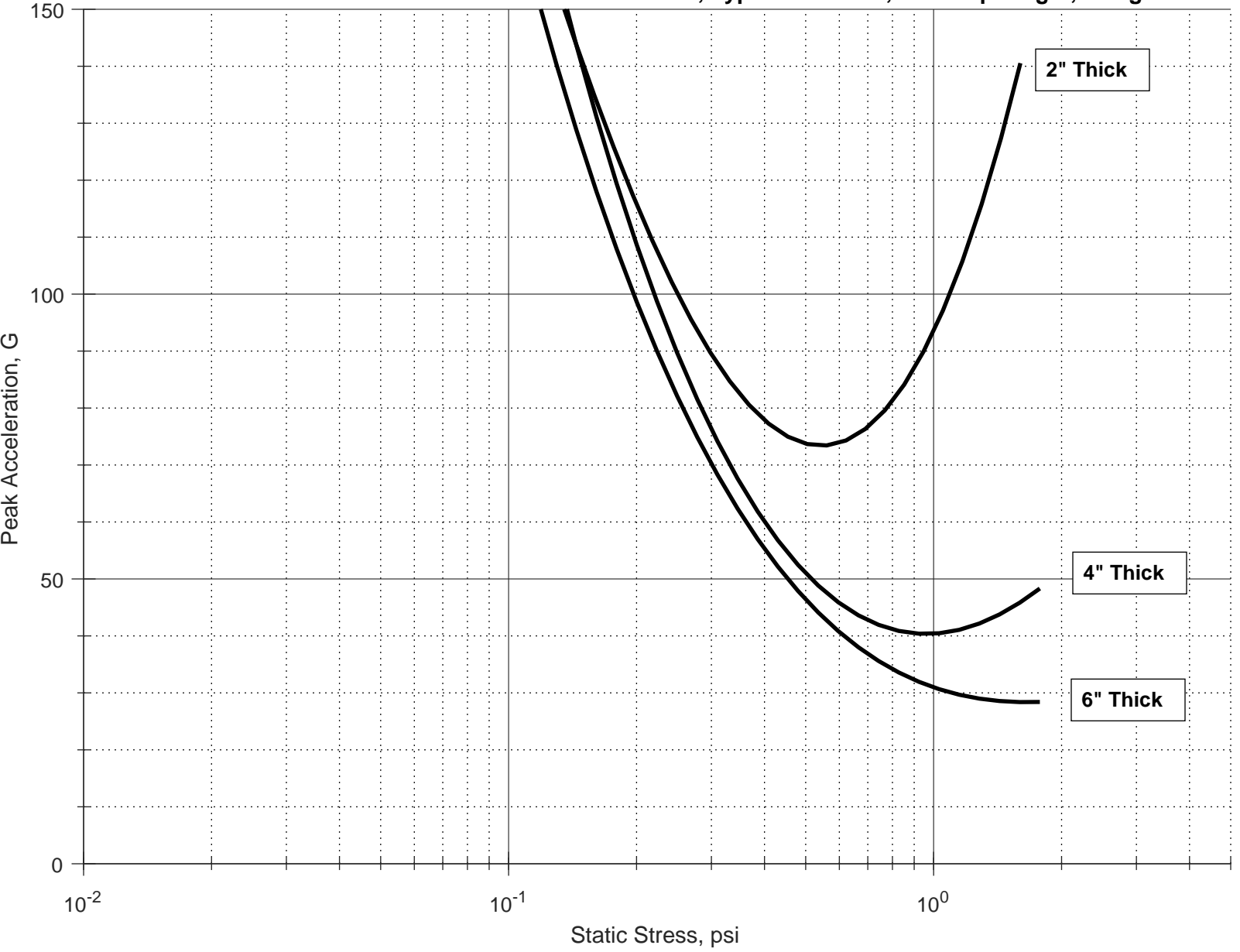
Peak Acceleration vs. Static Stress, Type 1 PE Foam, 36" Drop Height, 0 deg F
