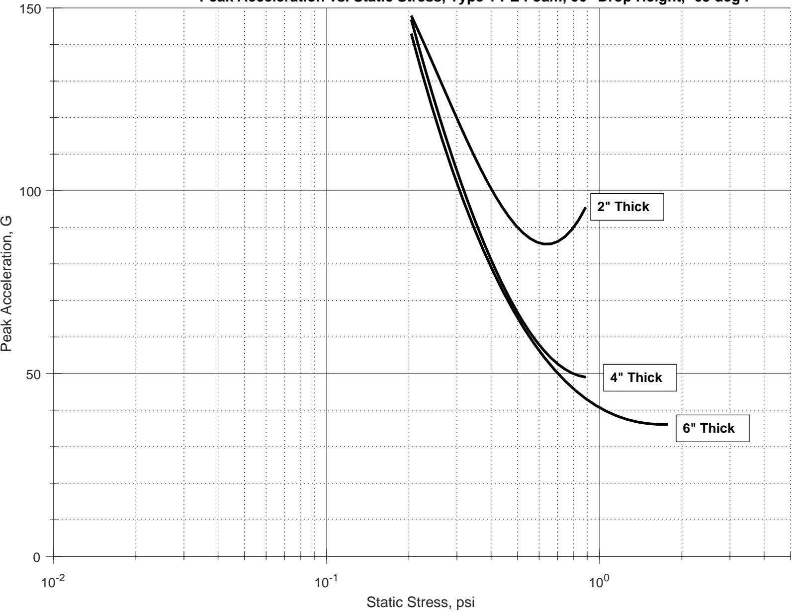
Peak Acceleration vs. Static Stress, Type 1 PE Foam, 36" Drop Height, -65 deg F
